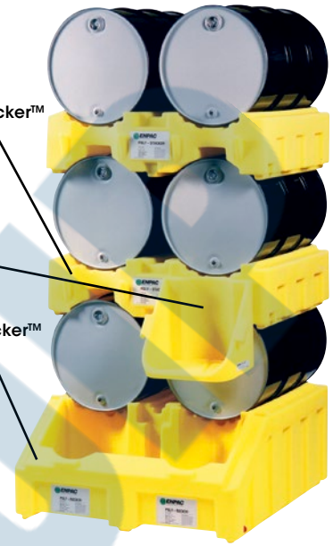
Multi-Purpose Racker/Stacker™
